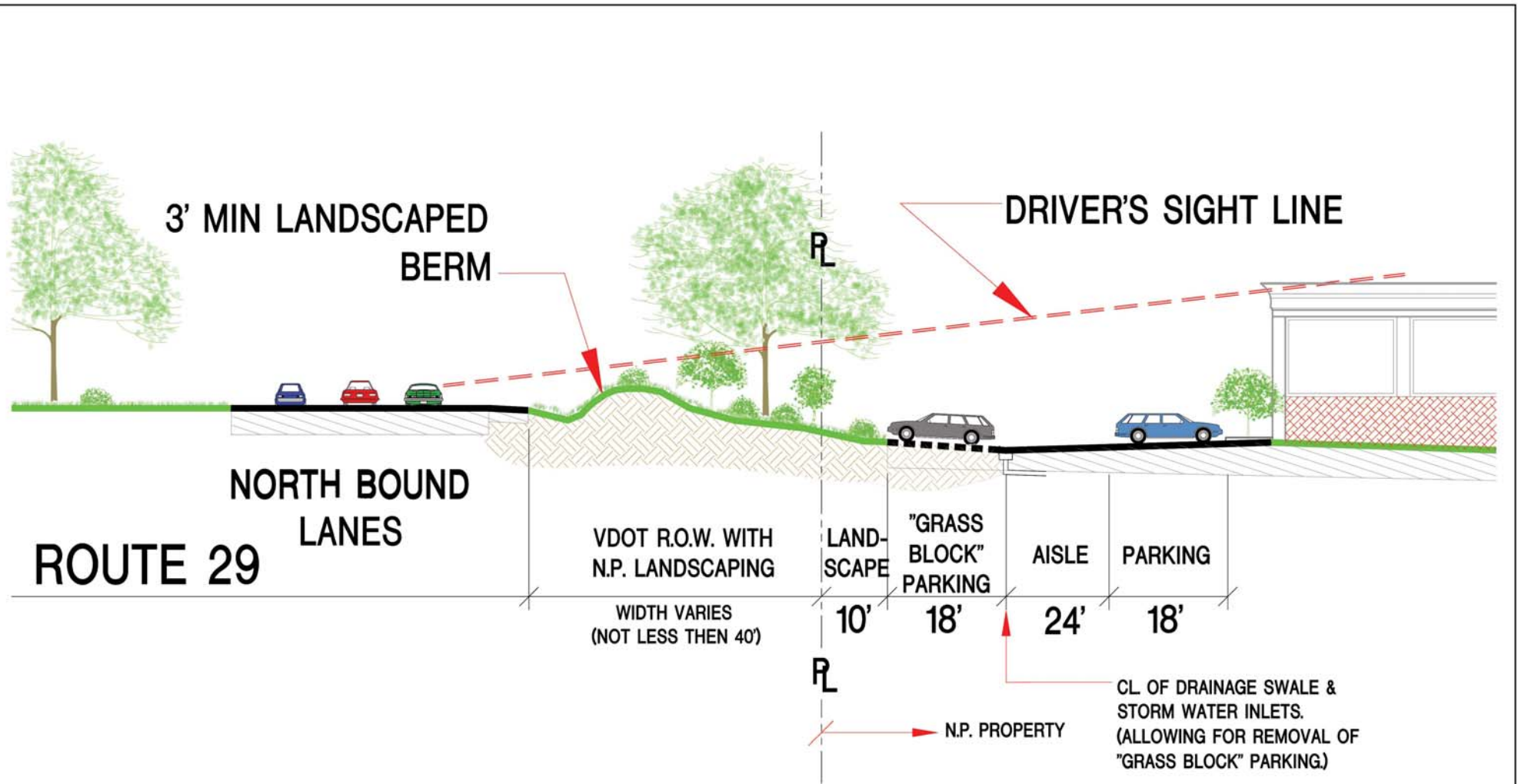
1 SS TYPICAL SITE SECTION of ROUTE 29 @ COMMERCIAL AREA LOOKING NORTH
